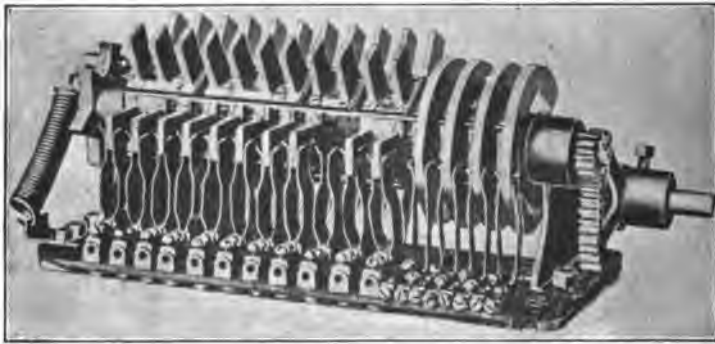
FIG. 445. —A Typical Electrical Vehicle Controller, or Circuit-Changing Switch. The circuit terminals of battery and motors are shown at the jack springs, which are arranged to be engaged by the fins on the periphery of the controller cylinder. The connections within the controller, between the fins, are, in general, the same as those shown in Fig. 448.
